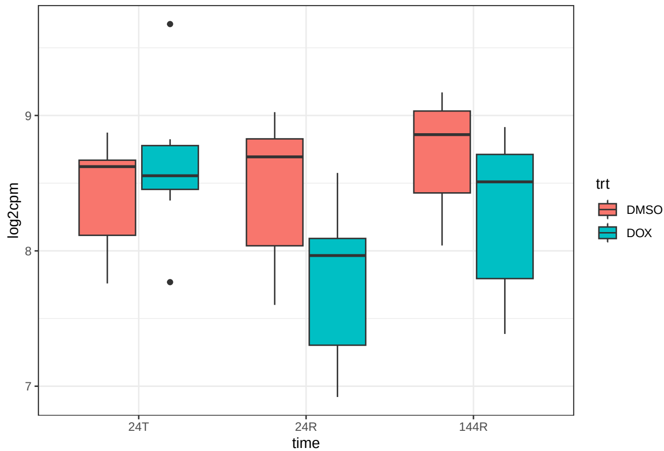
gene 51776 MAP3K20 dist 23198
